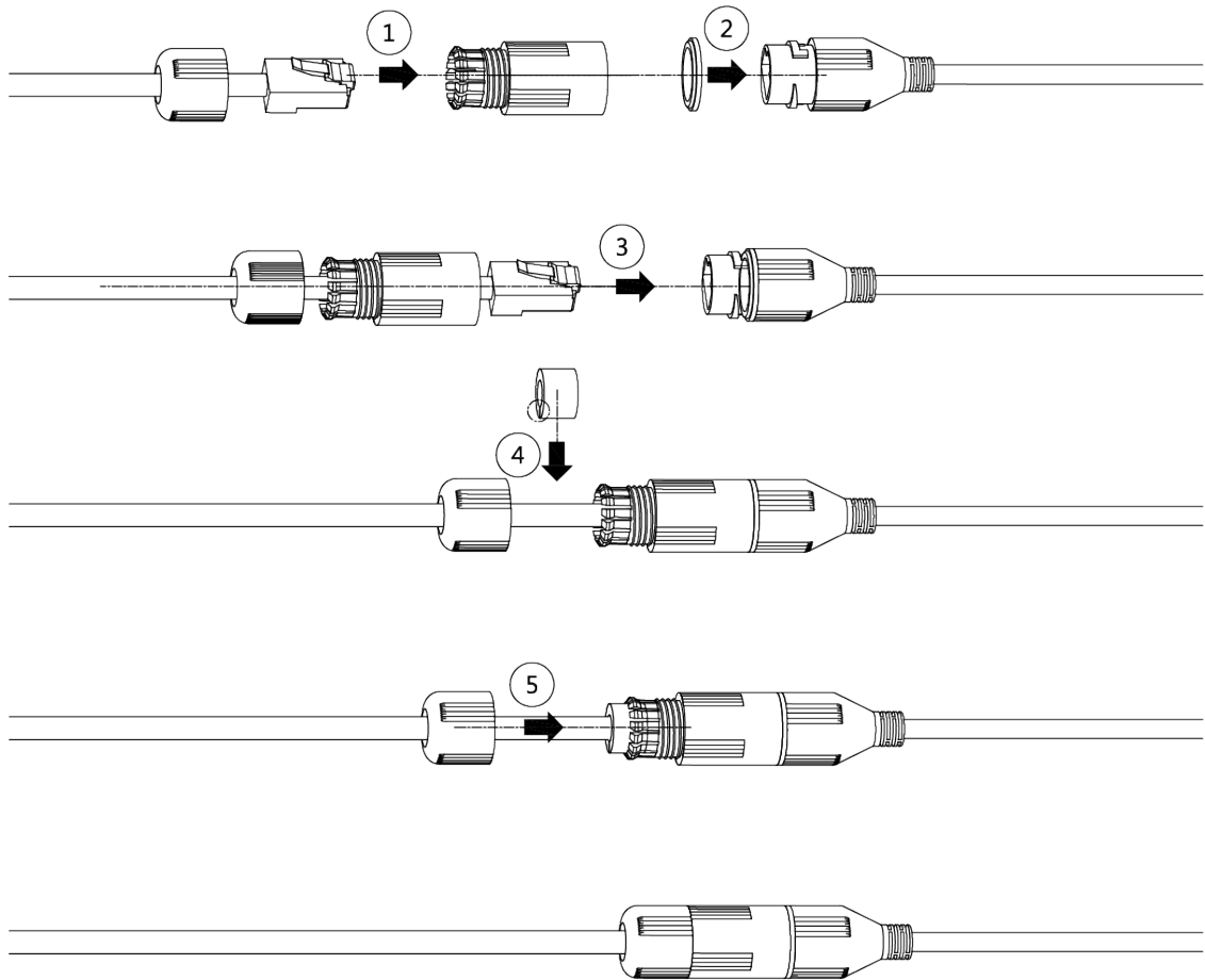
Figure 3-7 Install waterproof connector
