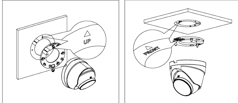
Figure 3-3 Installation direction
