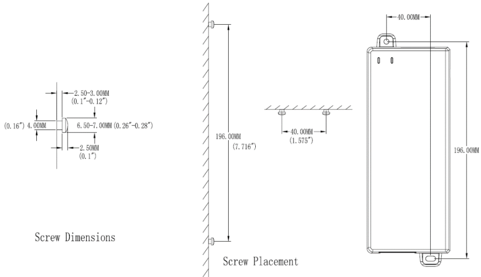
Figure 3-1 Wall mount
