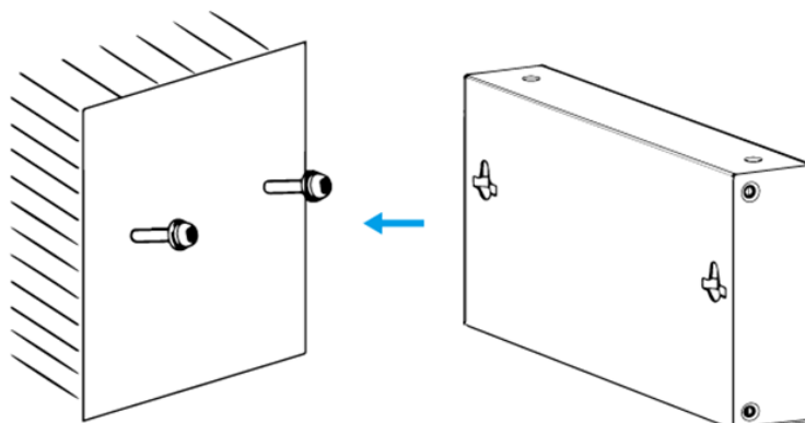
Figure 3-1 Wall mount
