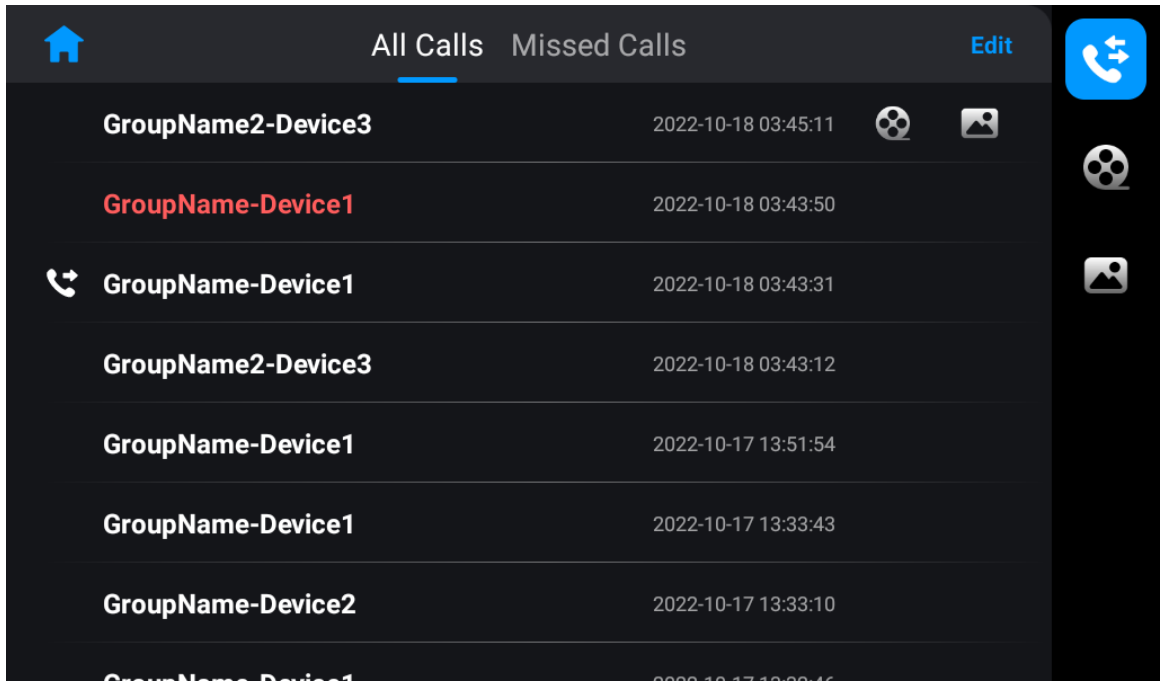
Figure 3-5 Call history
