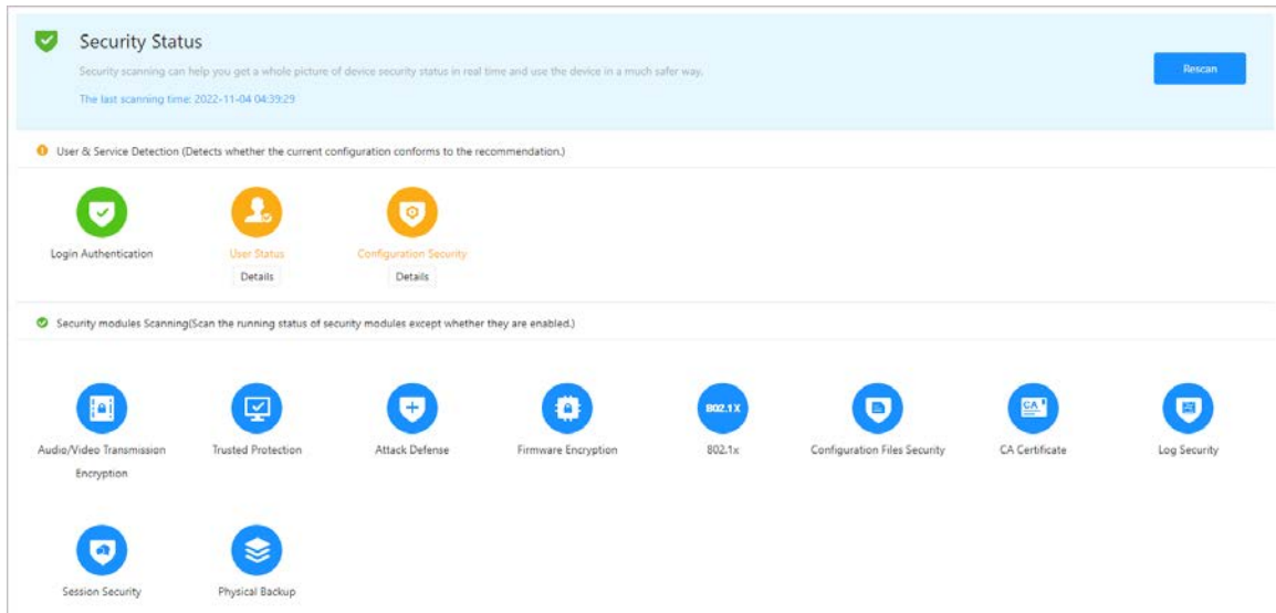
Figure 2-39 Security status
