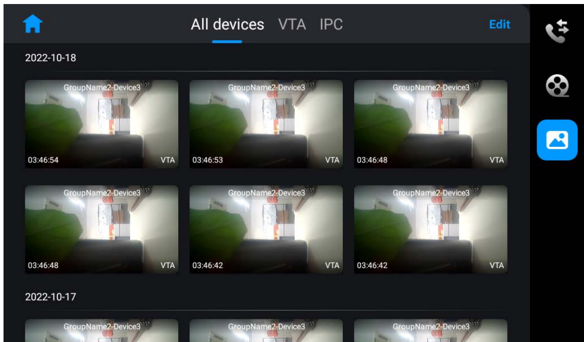
Figure 3-7 Snapshot files
