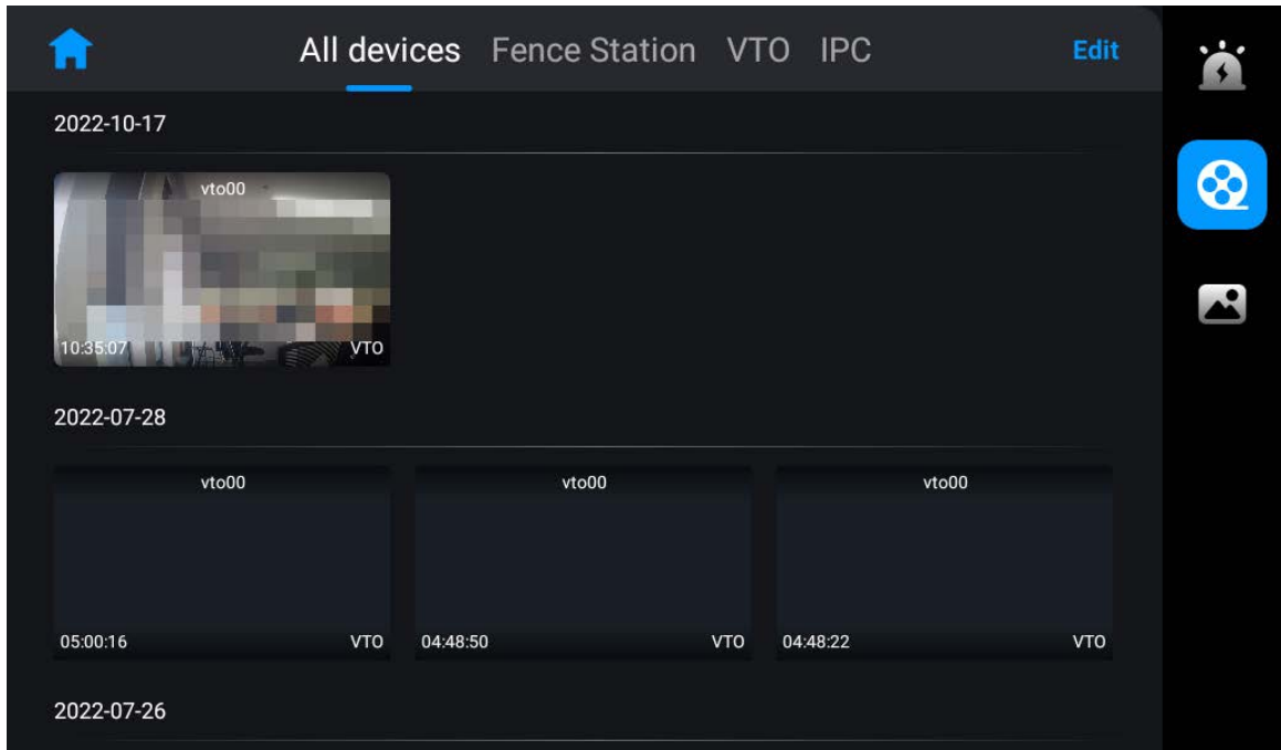
Figure 2-16 Video files
