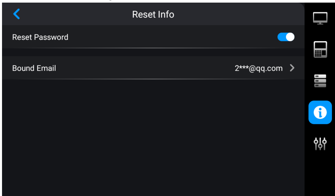
Figure 2-11 Reset information
