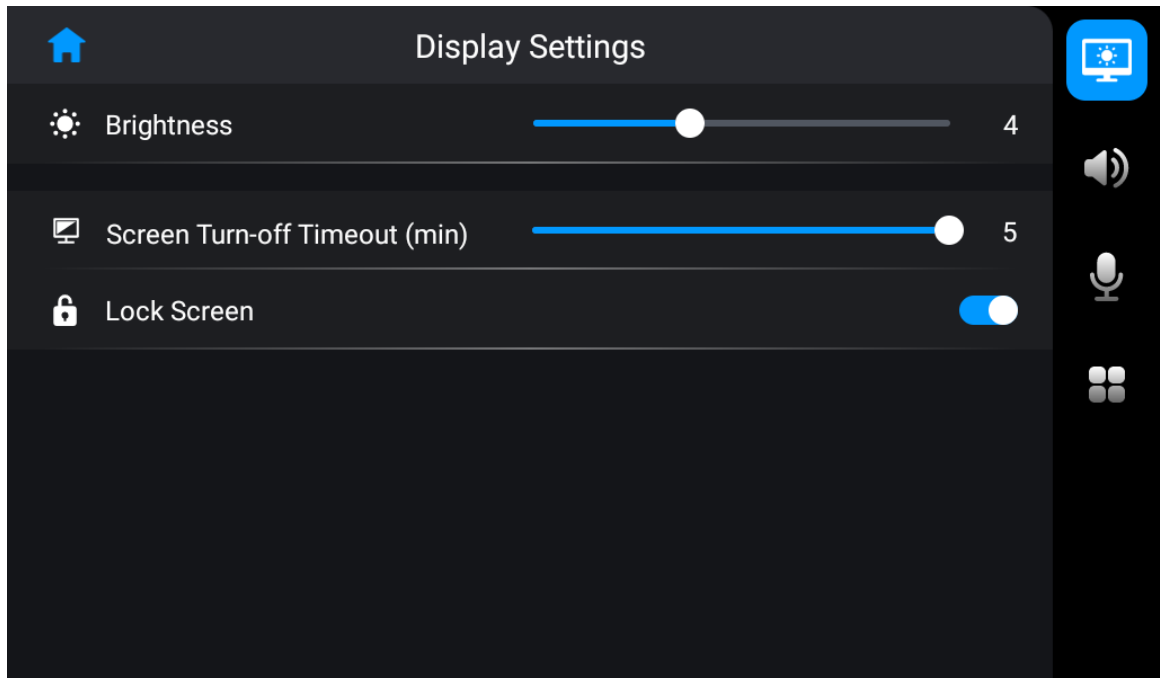
Figure 2-2 Display settings
