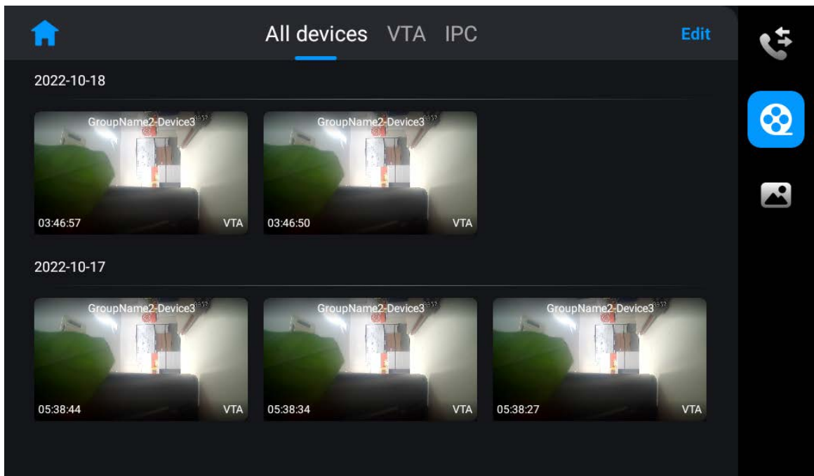
Figure 3-6 Video files
