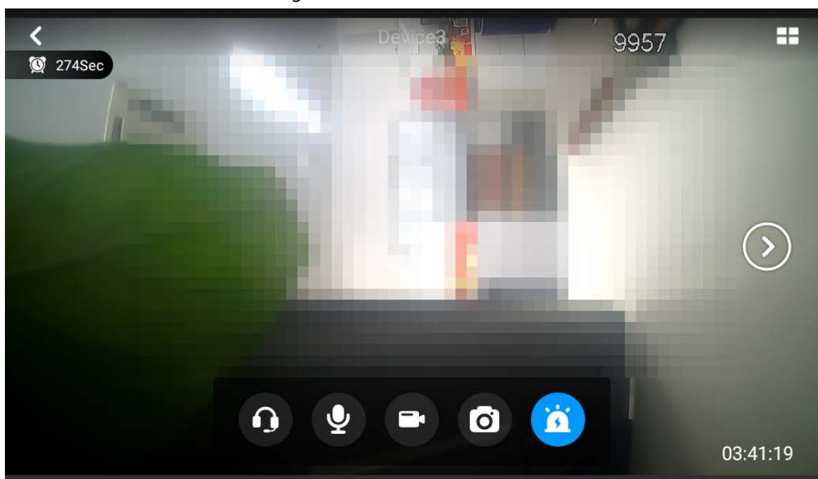
Figure 3-8 Monitor VTA
