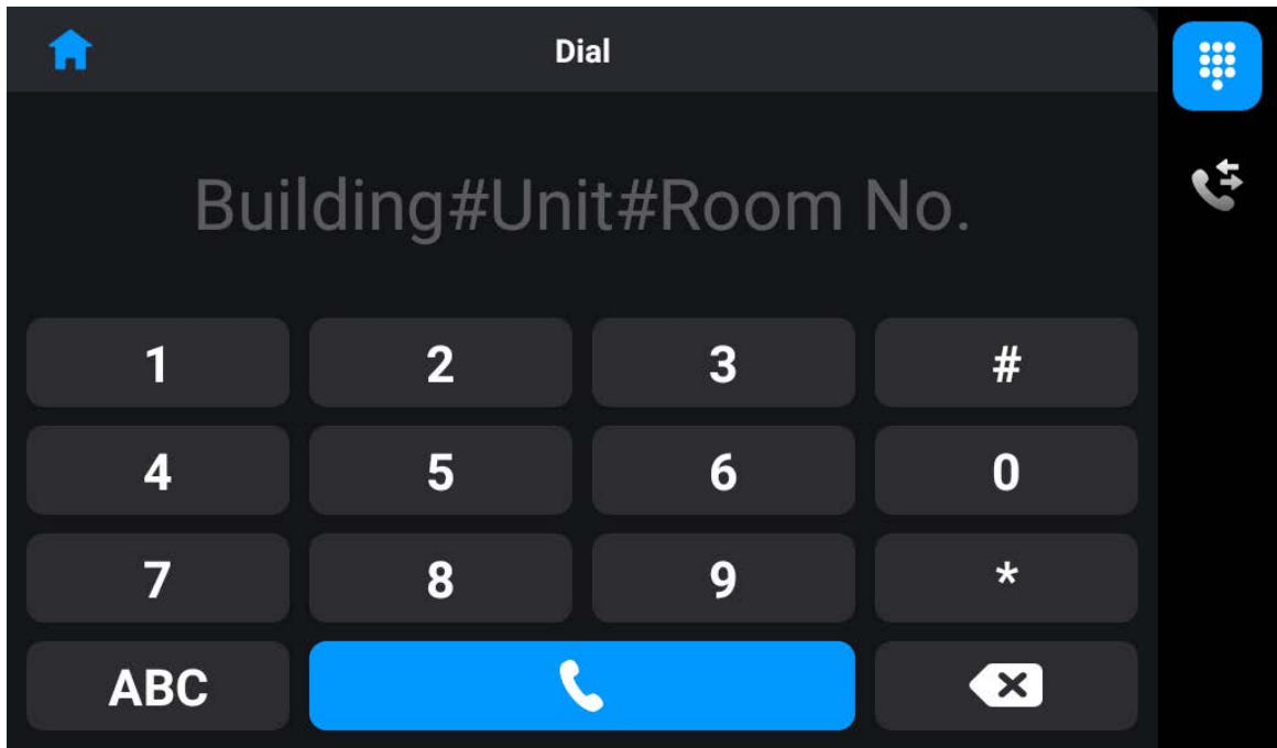
Figure 2-14 Call VTH
