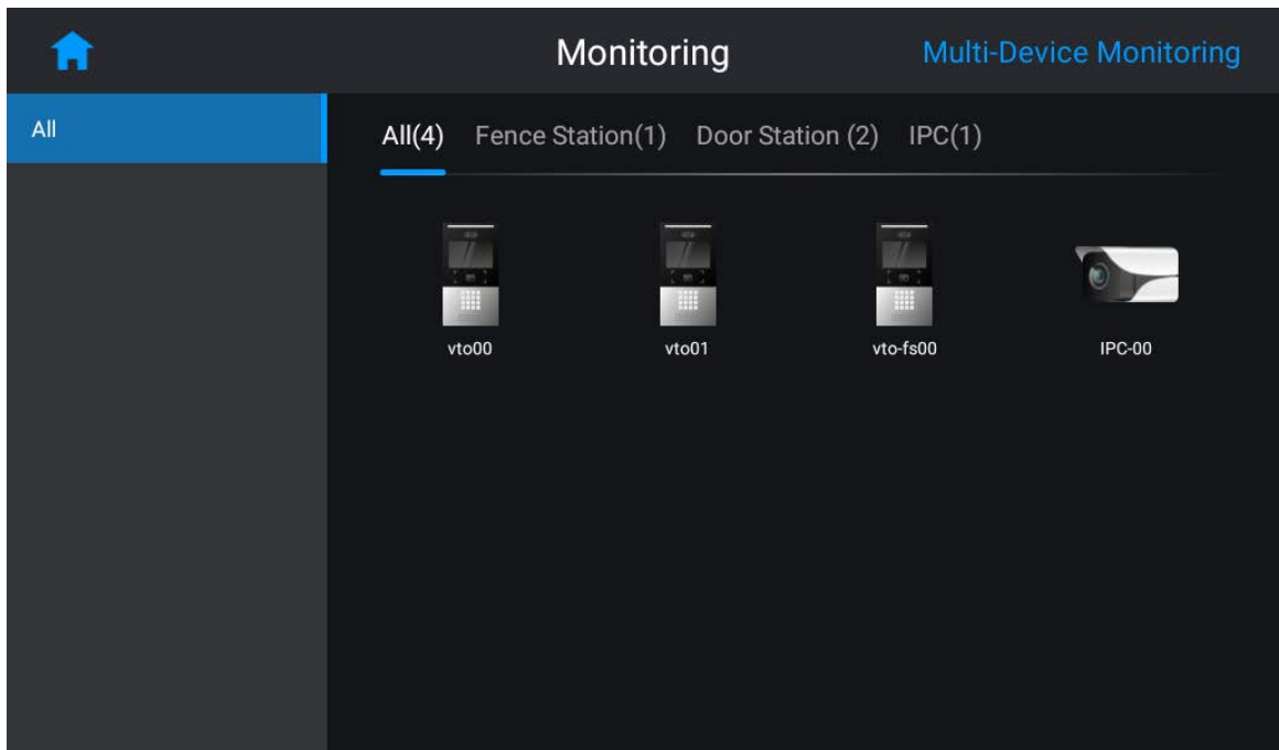
Figure 2-18 Select VTO
