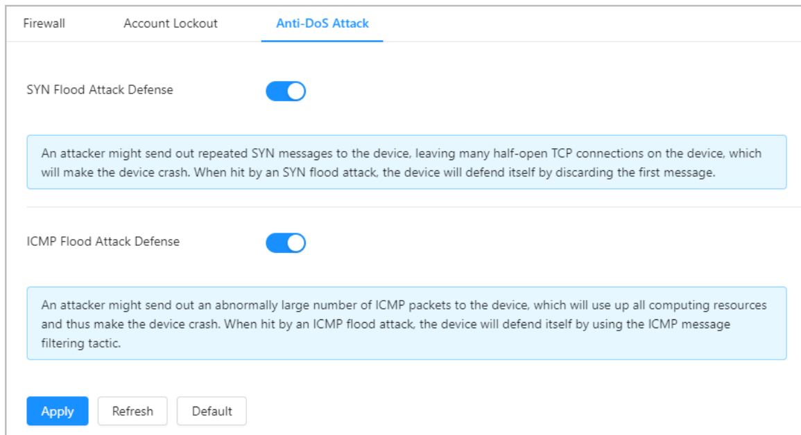
Figure 2-44 Anti-DoS Attack
