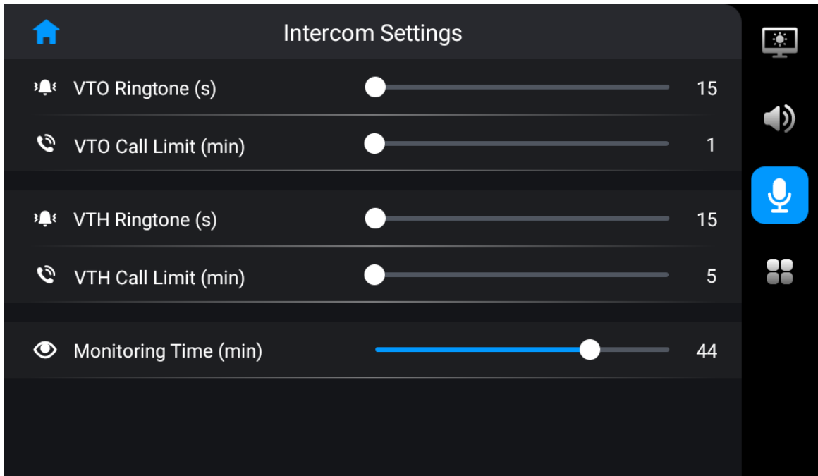
Figure 2-4 Intercom settings
