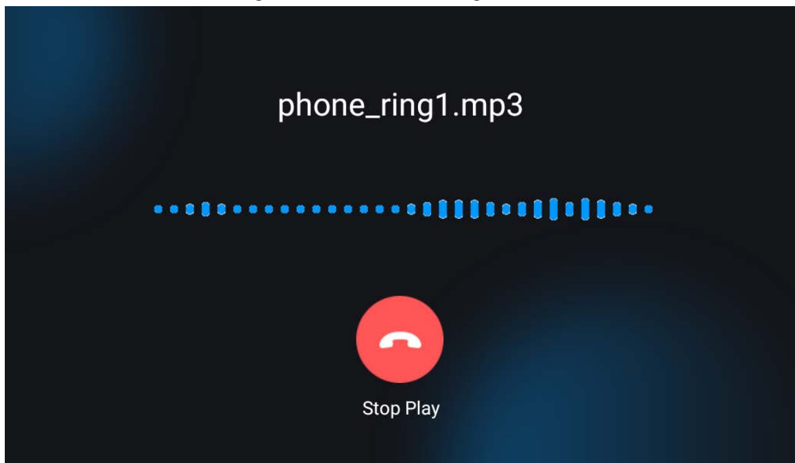
Figure 3-3 Audio broadcasting
