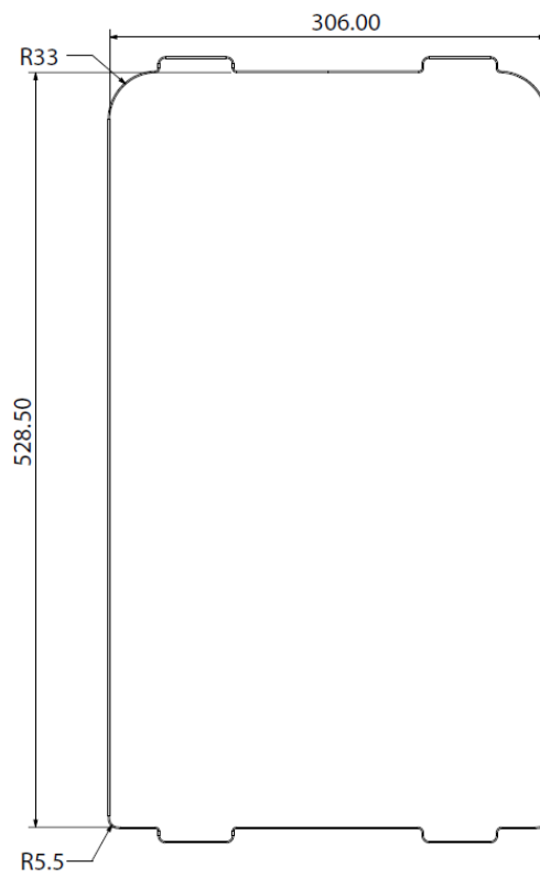
Advertising board dimensions (mm)
