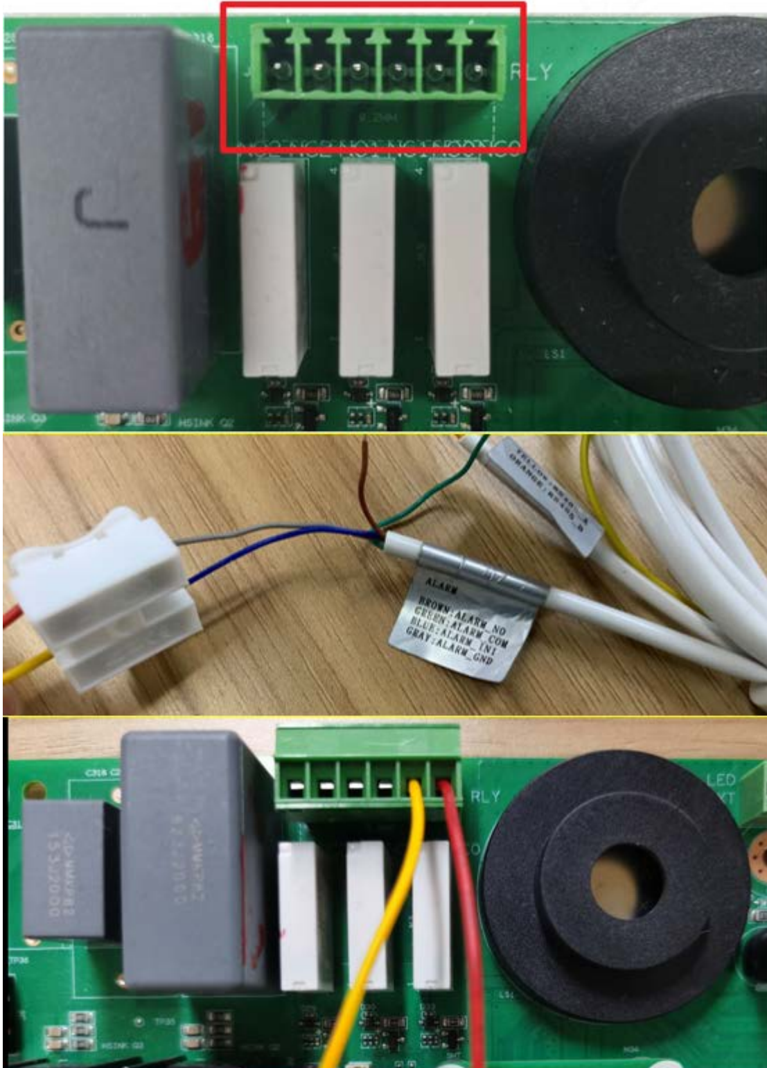
Alarm linkage cable connection
