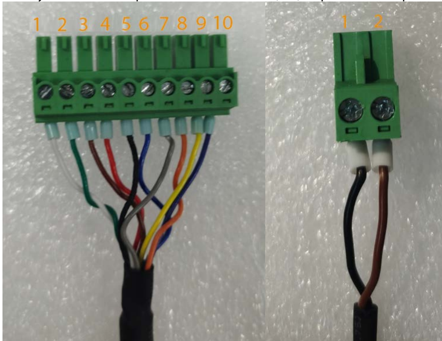
Primary antenna and replica antenna terminals (left)/Replica antenna power cable (right)
