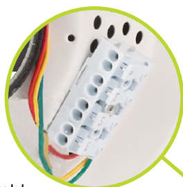
Spring loaded connection terminal
