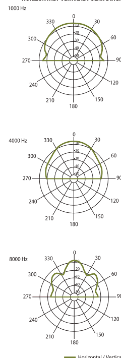
HORIZONTAL / VERTICAL POLAR DIAGRAMS
