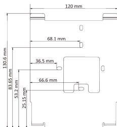
Figure 3-3 Mounting Plate
