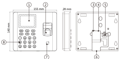
Figure 2-1 Device Appearance
