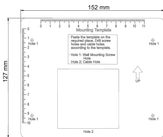
Figure 3-1 Mounting Template
