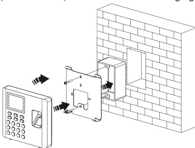
Figure 3-4 Install Device
