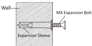
Figure 3-2 Install Screws
