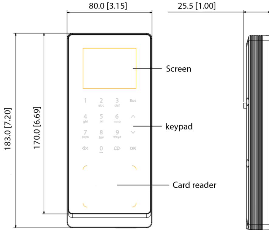
Figure 1-2 Dimensions (2) (mm[inch])
