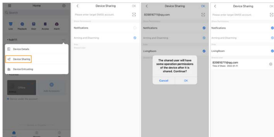
Figure 5-3 Share device
