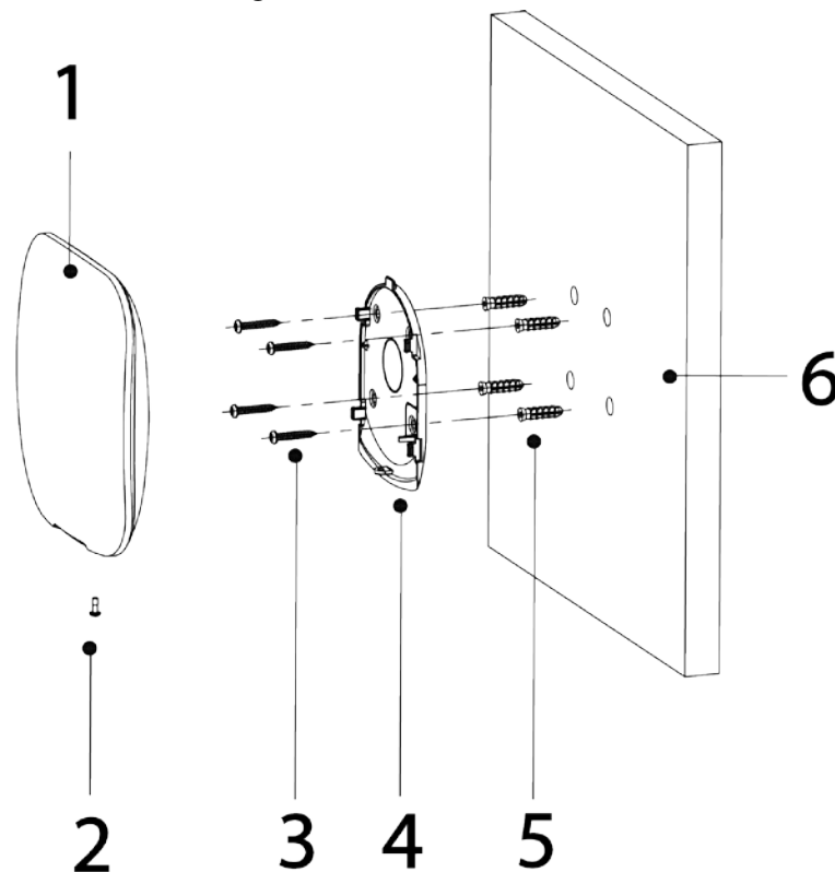
Figure 3-5 Installation
