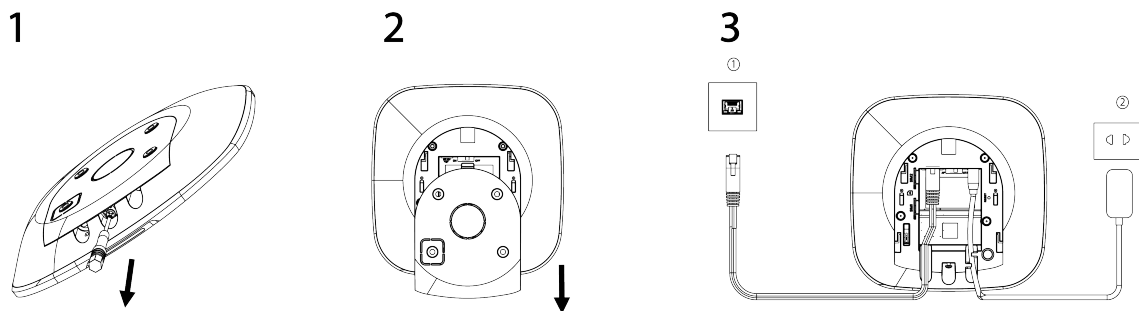
Figure 3-4 Power on
