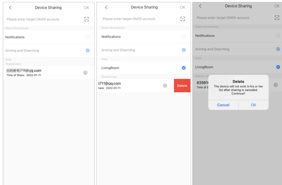
Figure 5-6 Share device
