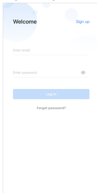
Figure 5-1 Login
