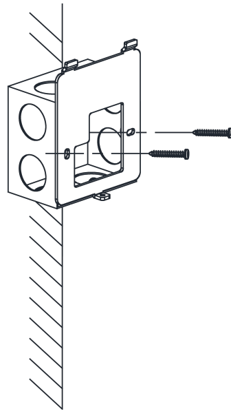
Figure 3-2 Install Mounting Plate
