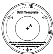
Figure 2-1 Drill Template
