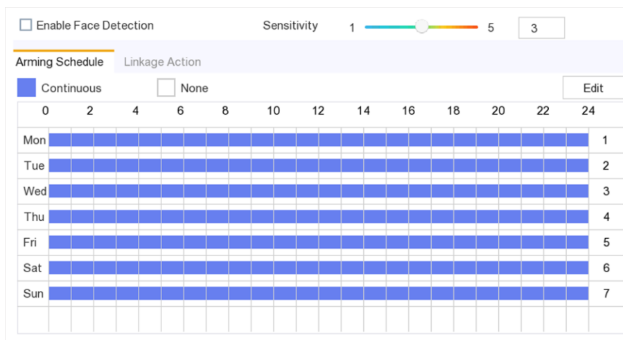
Figure 6-18 Face Detection
