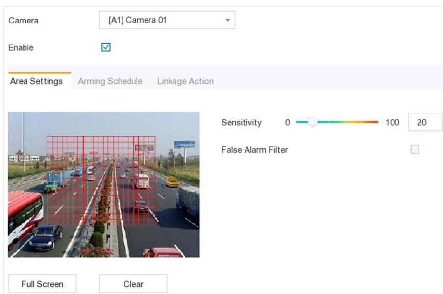
Figure 6-12 Motion Detection
