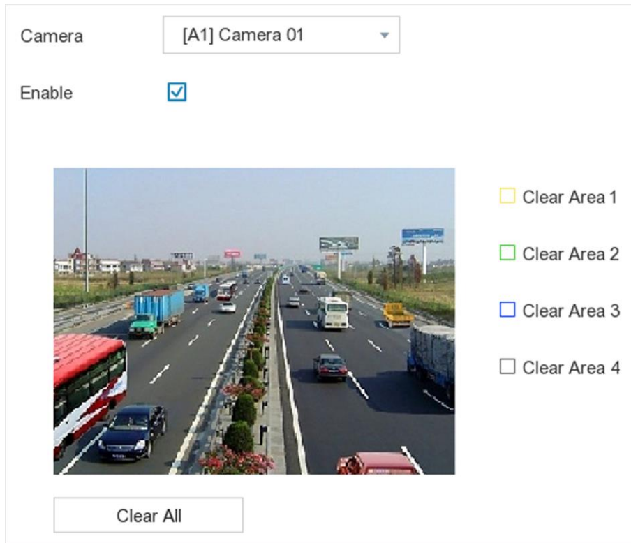
Figure 6-11 Privacy Mask
