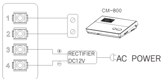
CM-801 terminal of backside
